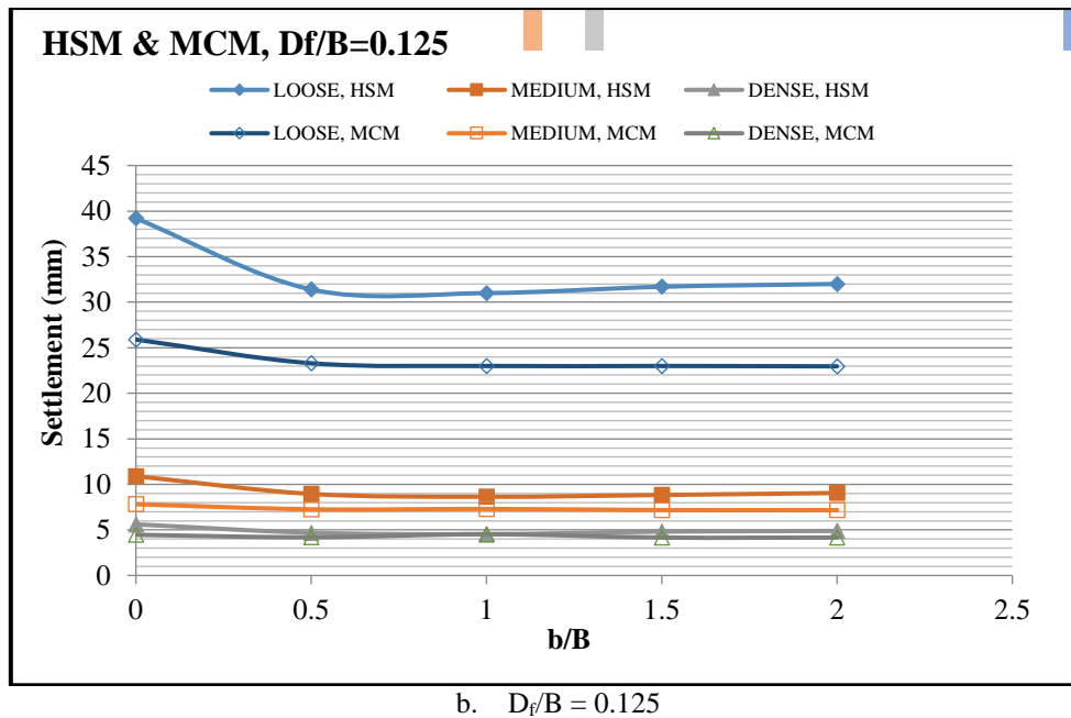
Figure 8. Maximum settlement in sand slope ( 30^\circ ) with different (b/B) ratio at different relative density of soil
