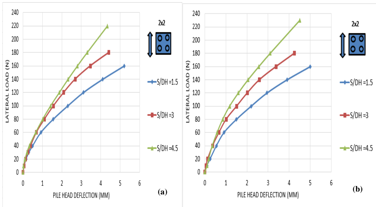
Figure 7. Load-lateral displacement curve for group (2x2), S (shaft pile spacing), Dh (helix diameter) (a) single helix, (b) double helix
