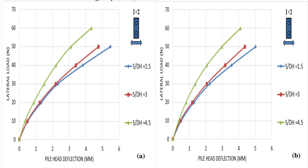
Figure 5. Load-lateral displacement curve for group (1x2), S (shaft pile spacing), Dh (helix diameter) (a) single helix, (b) double helix
