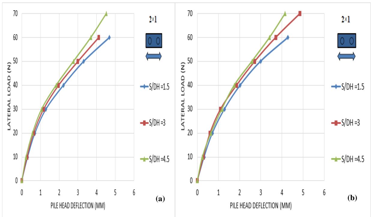
Figure 6. Load-lateral displacement curve for group (2x1), S (shaft pile spacing), Dh (helix diameter) (a) single helix, (b) double helix
