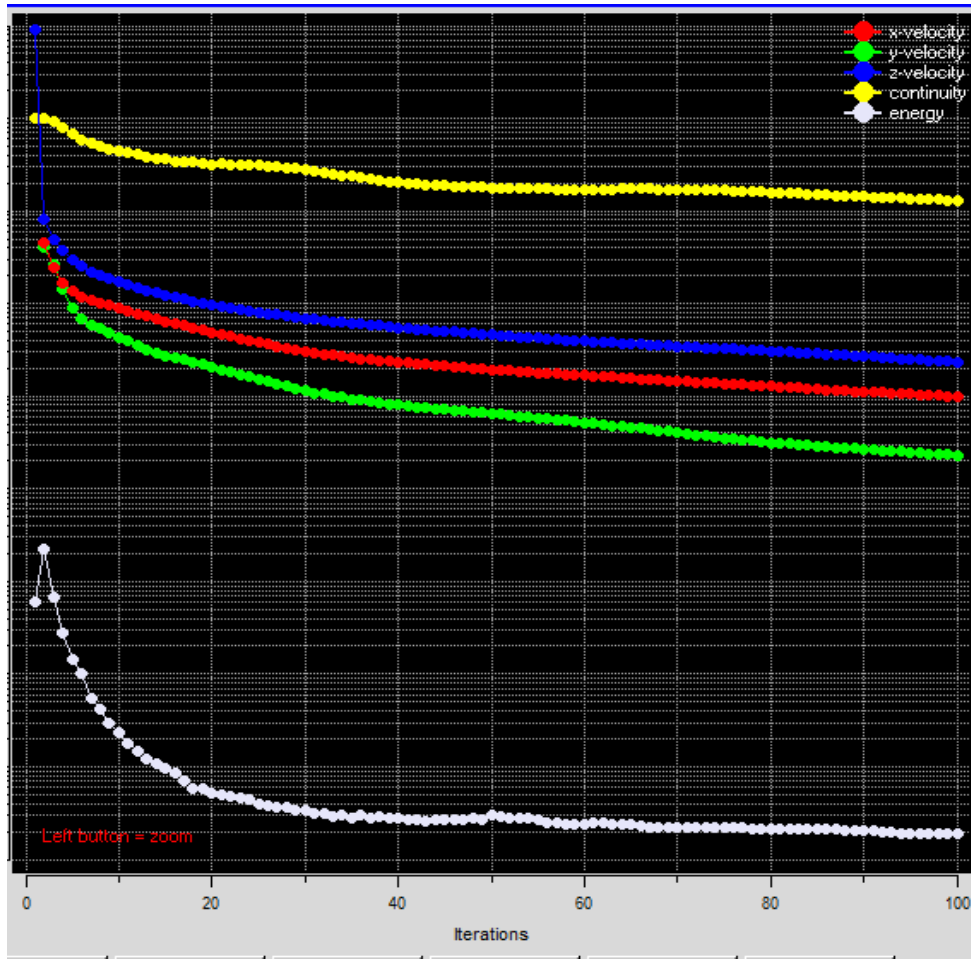
Figure (3) the residual of the operation at volumetric flows at 0.05\text{m}^3/\text{s} .
