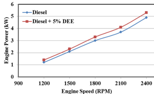
Figure 2: The trend of change of engine power with increasing speed
