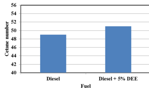
Figure 1: Effect of diethyl ether additive on fuel cetane number
