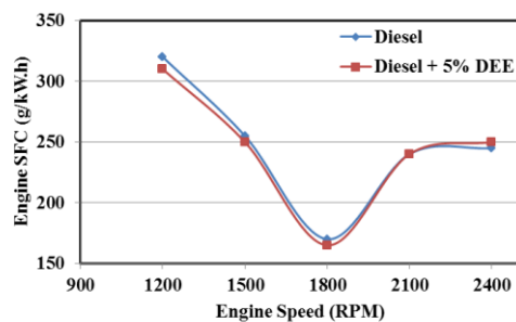
Figure 3: The trend of change of engine SFC with increasing speed
