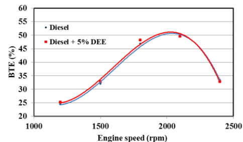
Figure 4: The trend of change of engine BTE with increasing speed
